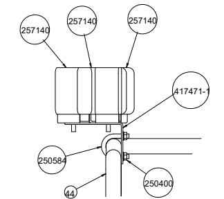
DETAIL S SCALE 1 : 4
