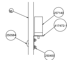
DETAIL T SCALE 1 : 4
