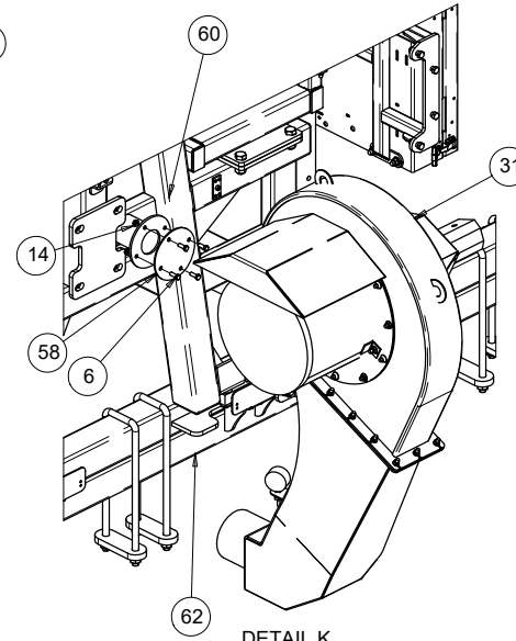
DETAIL K SCALE 1 : 16
