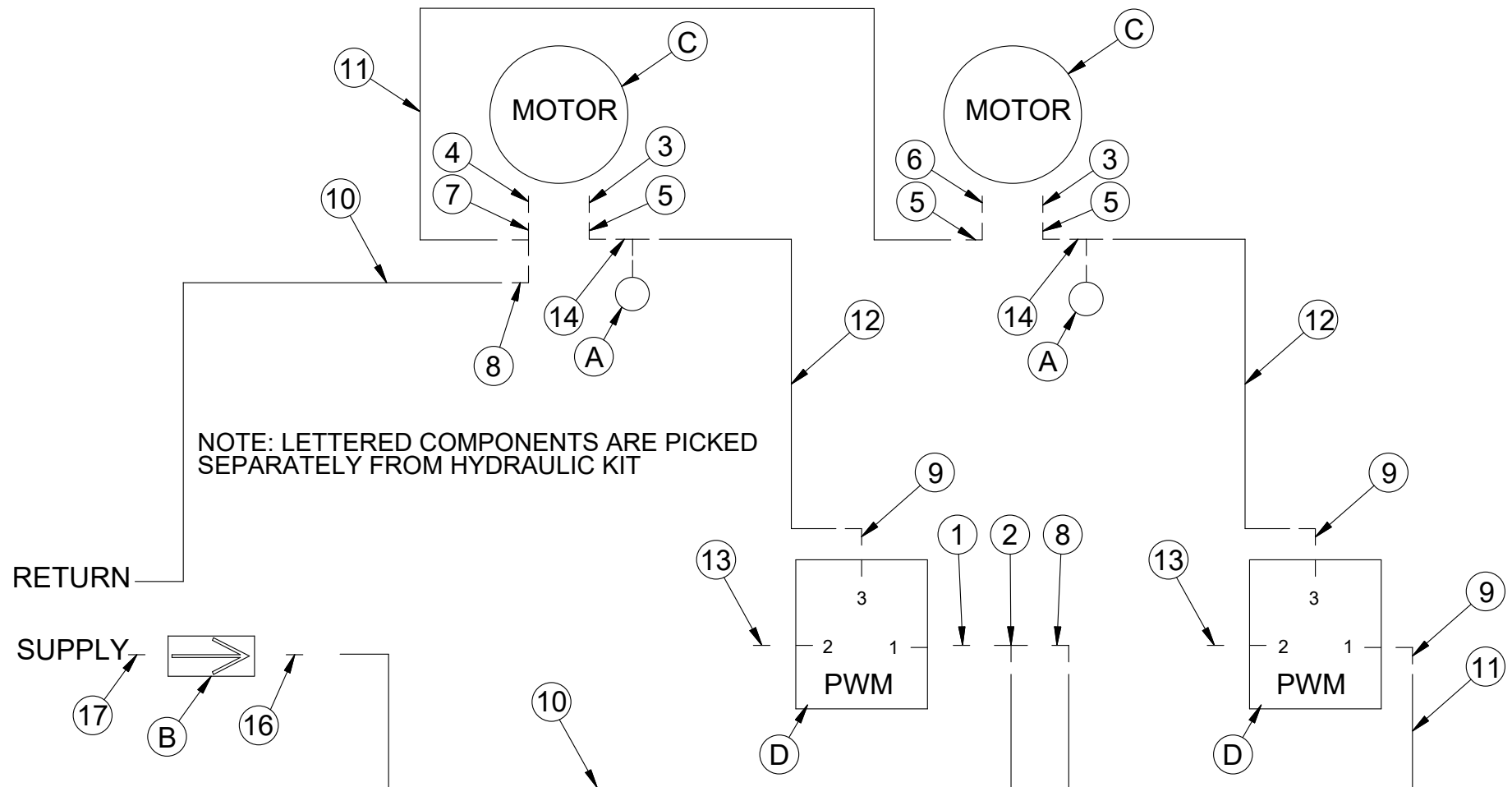
Meter Drive Schematic UltraPro II 360 BU Tank
