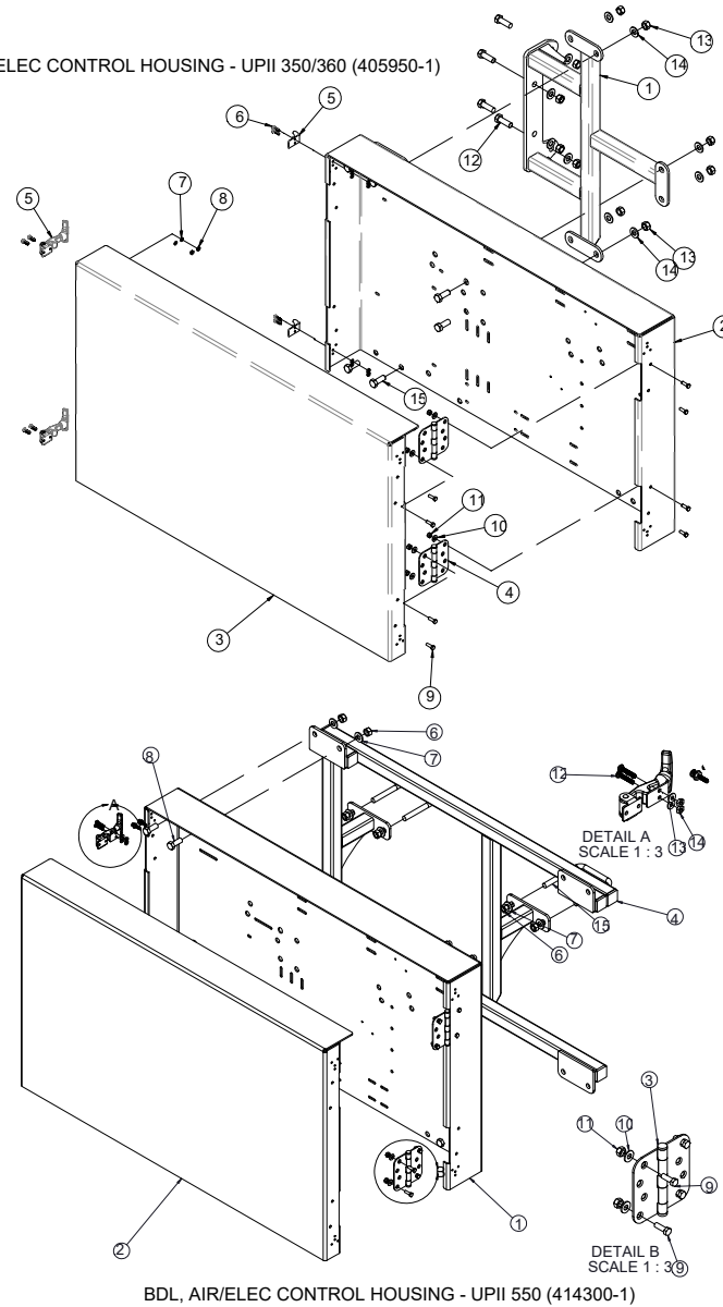
BDL, AIR/ELEC CONTROL HOUSING - UPII 550 (414300-1)
