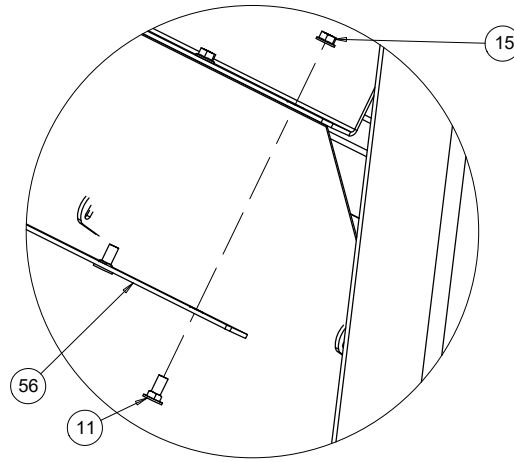
DETAIL H SCALE 1 : 4
