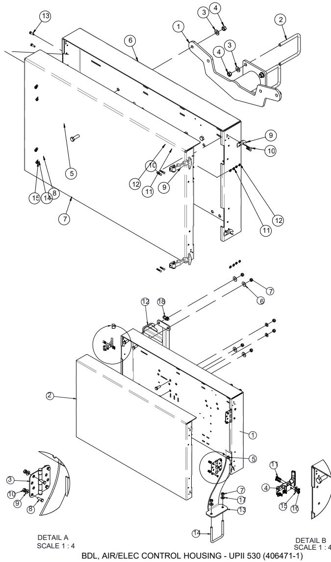
BDL, AIR/ELEC CONTROL HOUSING - UPII 20 (502502-2)
