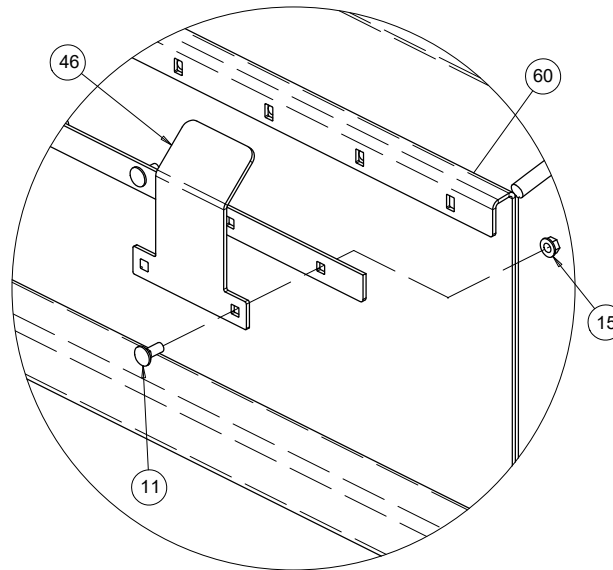
DETAIL J SCALE 1 : 4
