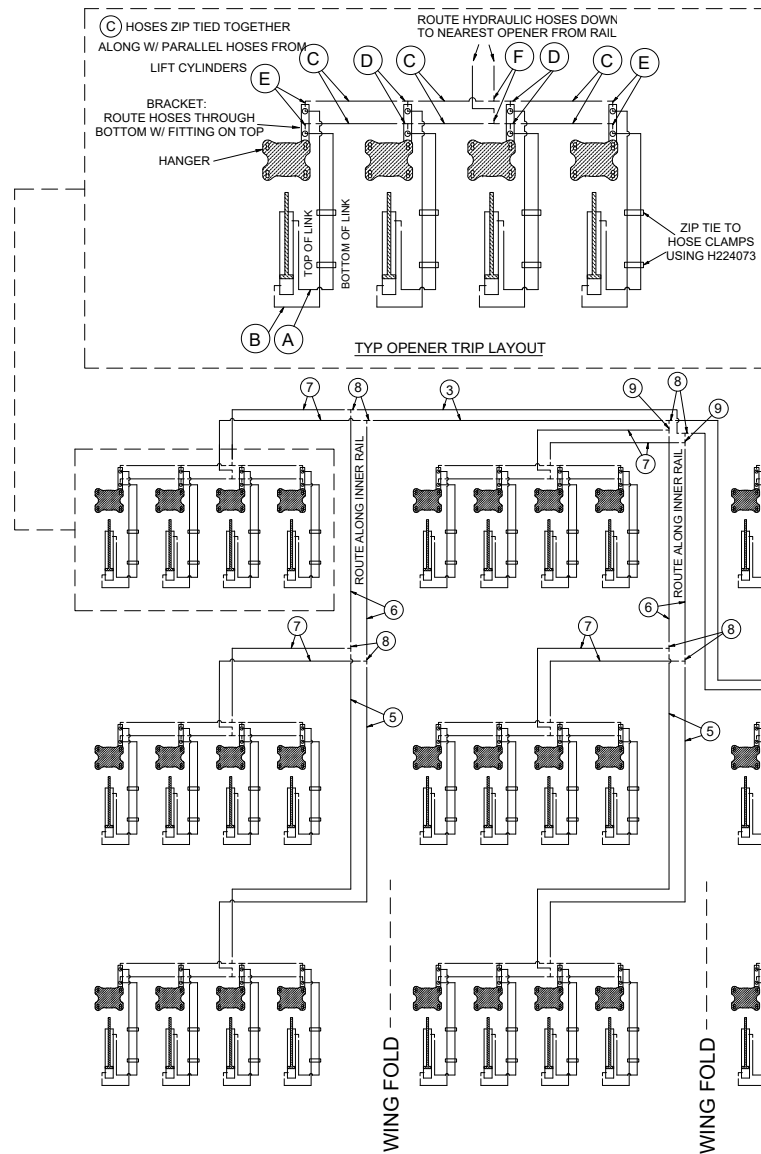
Opener Trip Hydraulic Schematic Part No. 421101
