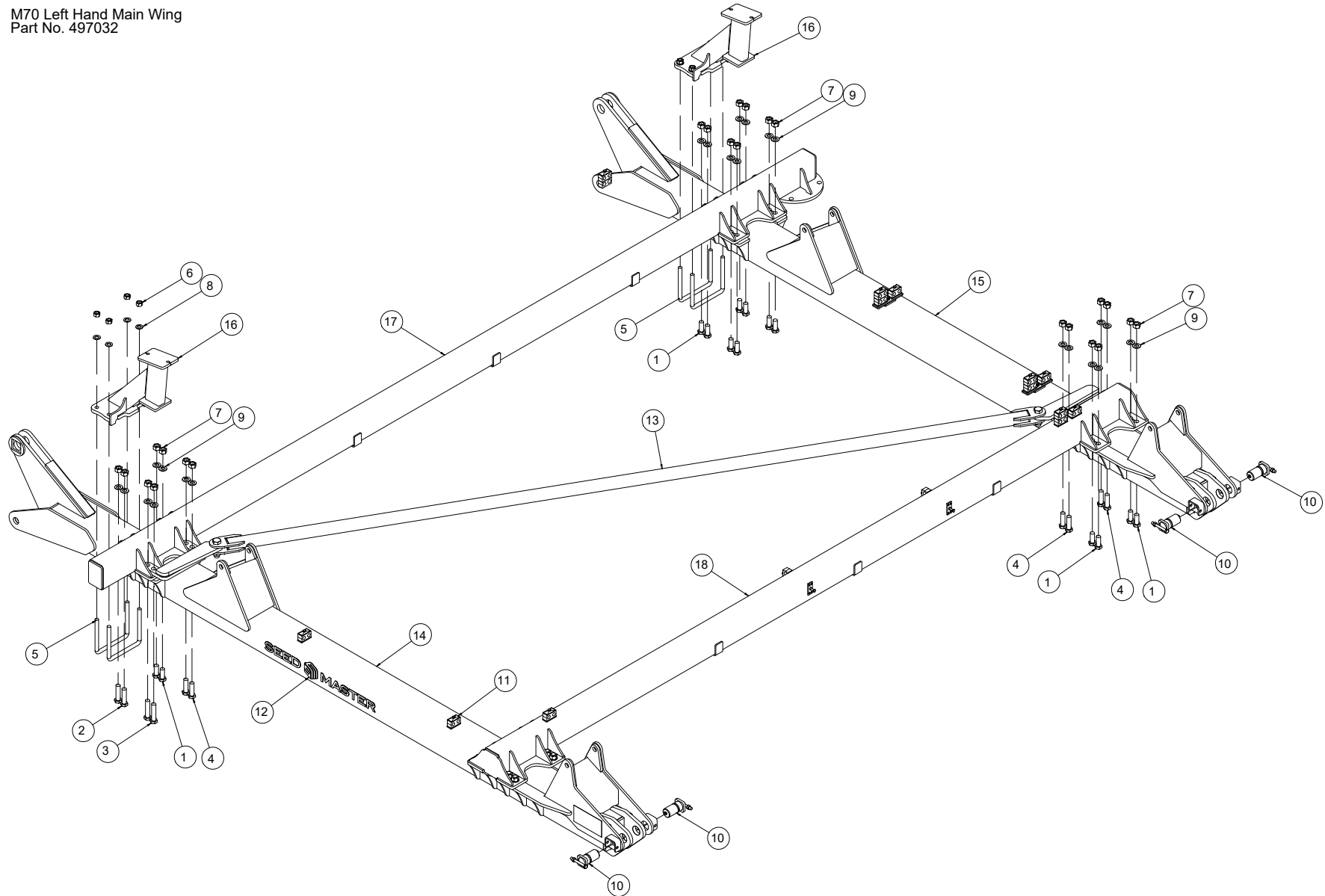
M70 Left Hand Main Wing
