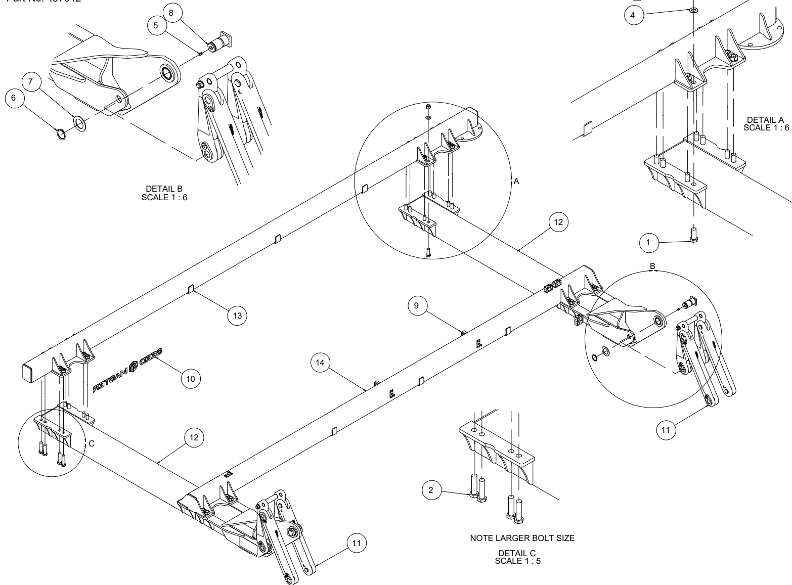
M80 Wide Left Hand Outer Wing Part No. 497042
