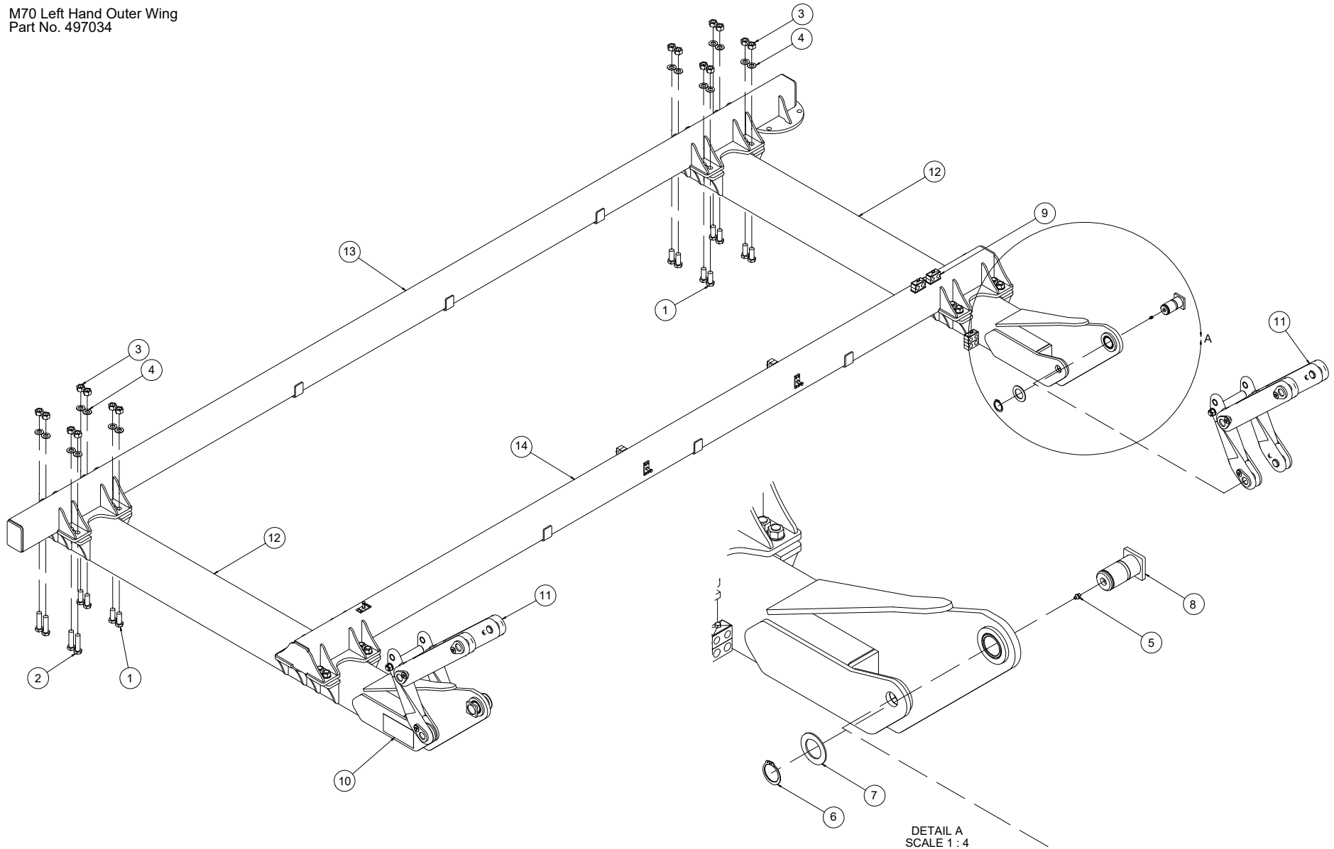
M70 Left Hand Outer Wing
