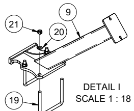
A407730 - WELD, WING STOP - MAIN - WIDE M80 - 40 3/8" - FRONT/REAR - BLK
