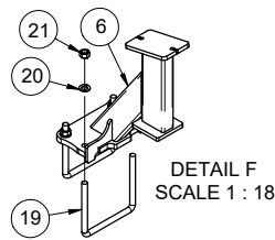
A407710 - WELD, WING STOP - FIFTH FOLD - M60 - BLK
