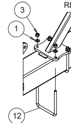
DETAIL P MAIN WING STOP TO REAR BEAM CONNECTION SCALE 1 : 20
