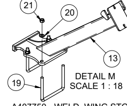
A407750 - WELD, WING STOP - MAIN - M90 - 43" - FRT - BLK
