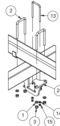
DETAIL K RANK TO WING RAIL CONNECTION
