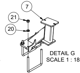
A407715 - WELD, WING STOP - FIFTH FOLD - M60 - BLK
