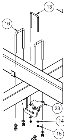
DETAIL A FIFTH FOLD WING STOP TO BEAM CONNECTION
