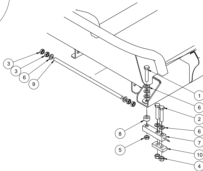
REAR ISOMETRIC EXPLODED VIEW
