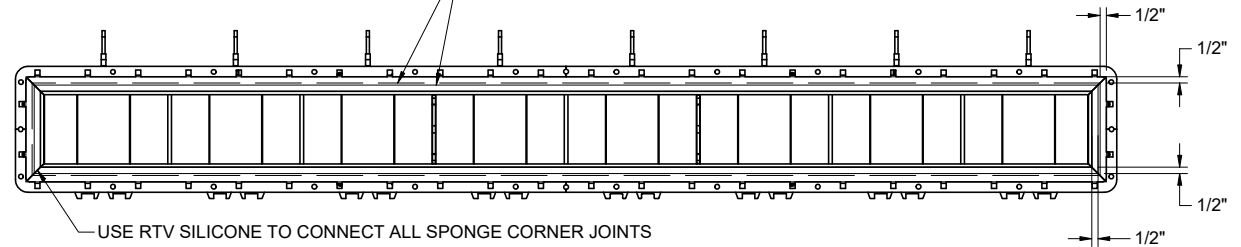
TOP VIEW
