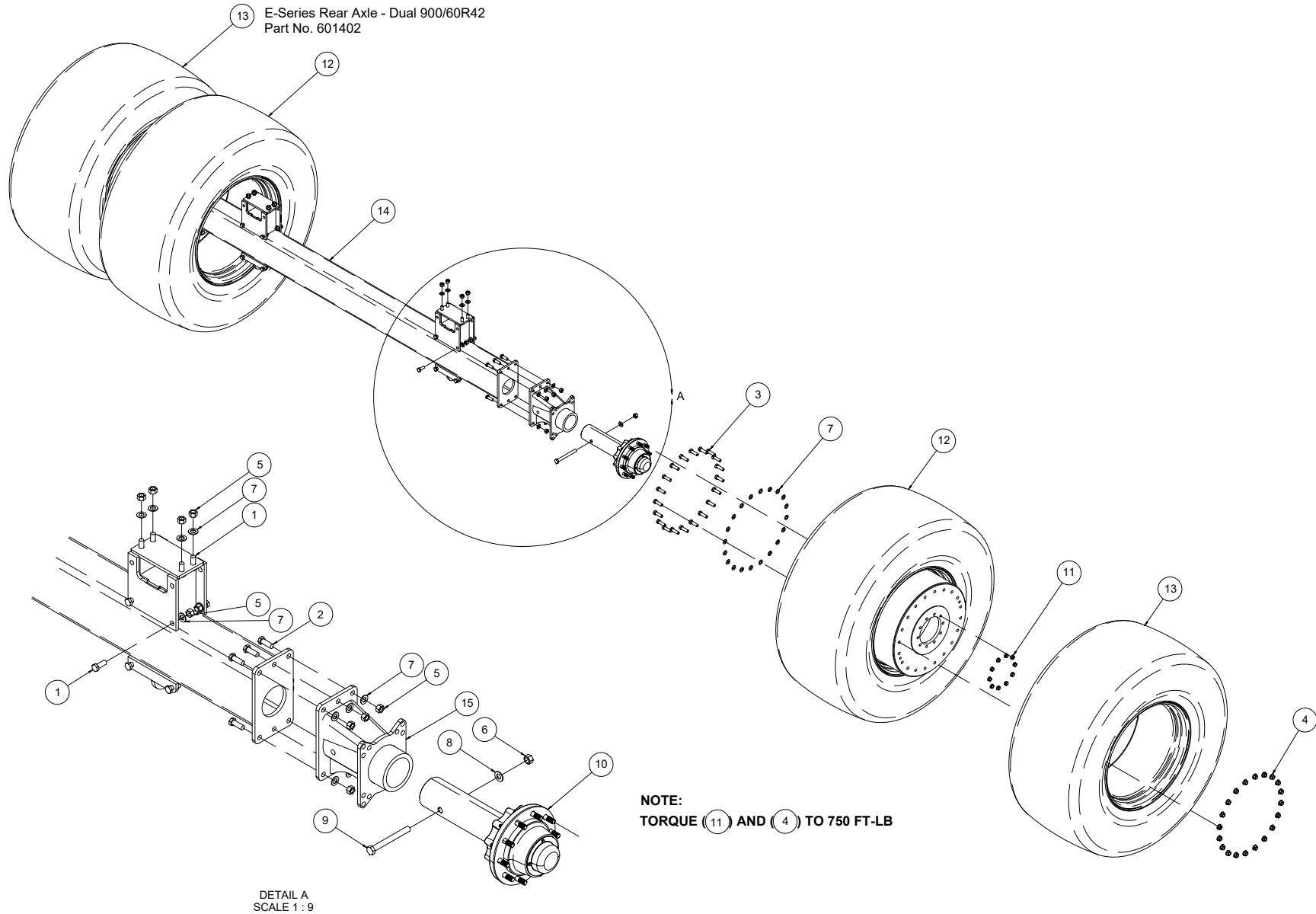
E860 Rear Axle - Dual 900/60R42
