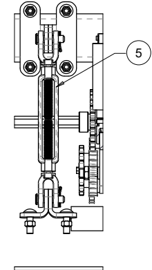
DETAIL BH SCALE 2 : 11
