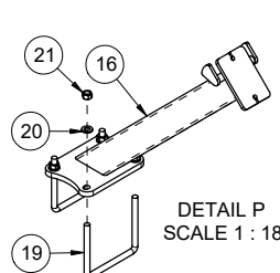
A407770 - WELD, WING STOP - MAIN - 40/50CT 3 PLEX - 40" - FRT - BLK
