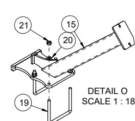
A407762 - WELD, WING STOP - MAIN - WIDE M WITH UPII550 - REAR - BLK
