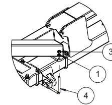
DETAIL E ANGLE BRACKET TO BEAM CONNECTION
