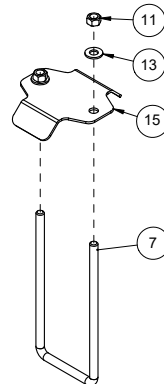
510302 BDL, HANGER - 2 PIPE- DISTRIBUTION
