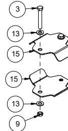
510358 BDL, HANGER - 2 PIPE - DISTRIBUTION
