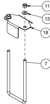
510482 - BDL, PIPE HOLDER - DISTRIBUTION - 6IN - 2 PIPE
