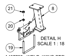
A407725 - WELD, WING STOP - FIFTH FOLD - M80CT - BLK
