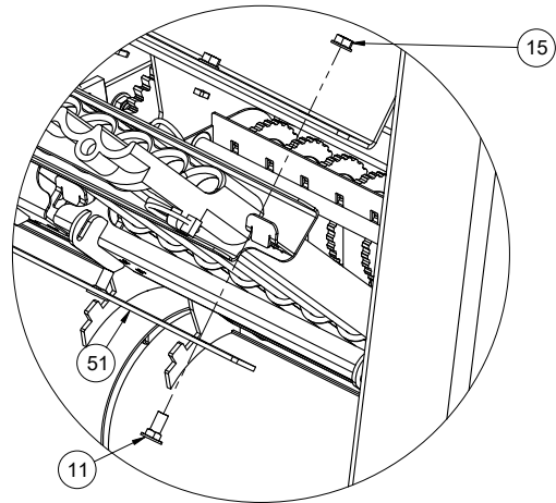
DETAIL H SCALE 1 : 4
