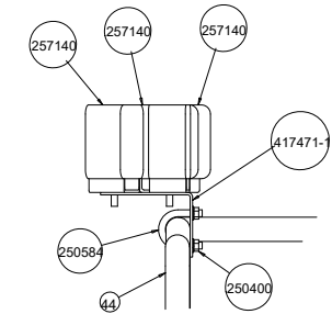
DETAIL S SCALE 1 : 4
