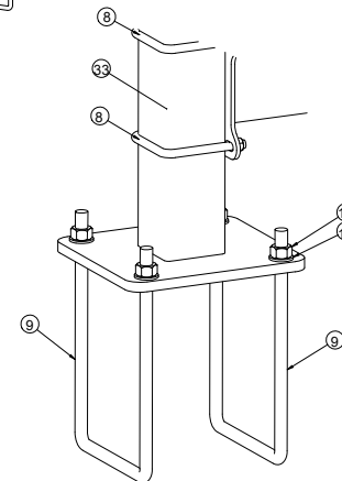
DETAIL C SCALE 1 : 4
