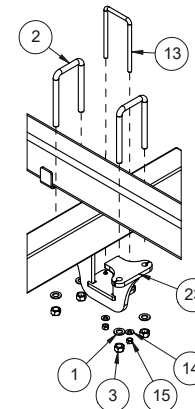
DETAIL K RANK TO WING RAIL CONNECTION
