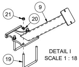
A407730 - WELD, WING STOP - MAIN - WIDE M80 - 40 3/8" - FRONT/REAR - BLK
