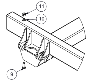
DETAIL F RAIL TO BEAM CONNECTION
