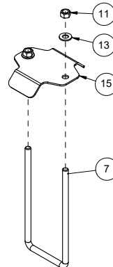
510302 BDL, HANGER - 2 PIPE- DISTRIBUTION
