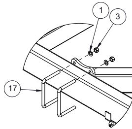
DETAIL C ANGLE BRACKET TO RAIL CONNECTION
