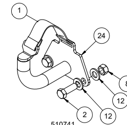
510741 BDL, PIPE HOLDER - DISTRIBUTION - 6IN - 2 PIPE
