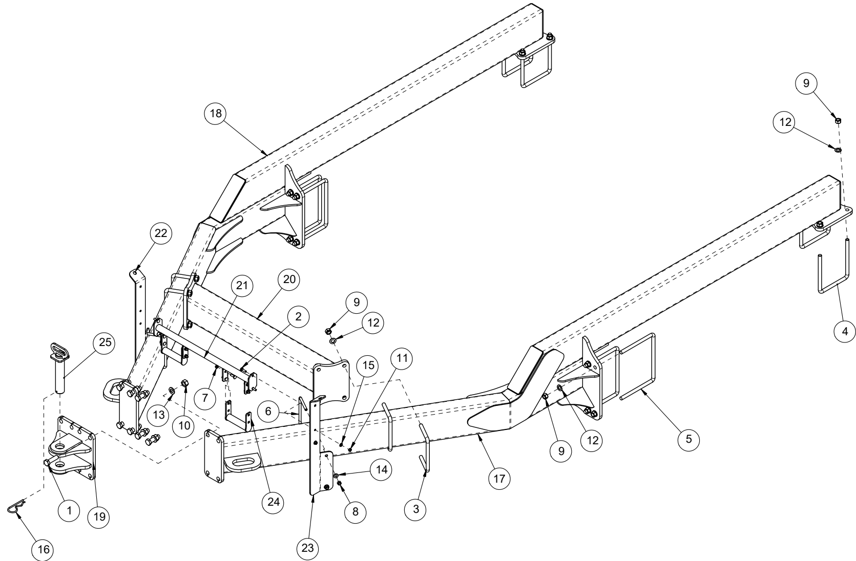
Rear Hitch - JD C850 - 12x8 Axle - Extended Rails
