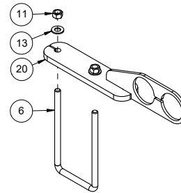
510483 - BDL, PIPE HOLDER - DISTRIBUTION - 2 PIPE
