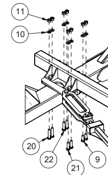
DETAIL L MAIN WING TO WINGBRACE REAR CONNECTION
