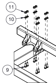
DETAIL M WING RAIL TO BEAM CONNECTION
