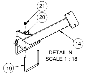
A407753 - WELD, WING STOP - MAIN - WIDE M WITH UPII550 - FRONT - BLK
