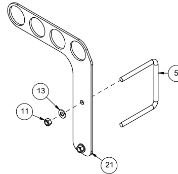
510484 BDL, PIPE HOLDER - DISTRIBUTION - 4 PIPE - OFFSET
