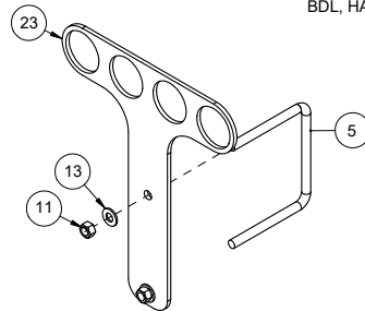
510486 - BDL, PIPE HOLDER - DISTRIBUTION - 4 PIPE - CENTER
