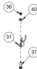
405372 - WELD, SINGLE HOSE BOLT ON CLAMP - BL
