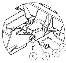
DETAIL B HINGE PIN CONNECTION
