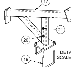
A407977 - WELD, WING STOP - STD 5 PLEX - REAR - BLK
