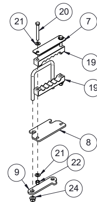
407266 - BAG, HDW - FRT HITCH HYD HOSE CLAMP- SEEDMASTE
