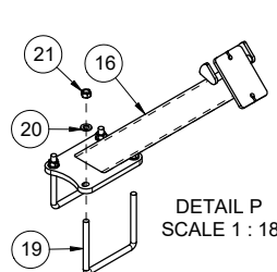
A407762 - WELD, WING STOP - MAIN - WIDE M WITH UPII550 - REAR - BLK
