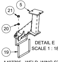
A407705 - WELD, WING STOP - FIFTH FOLD - M50 - BLK
