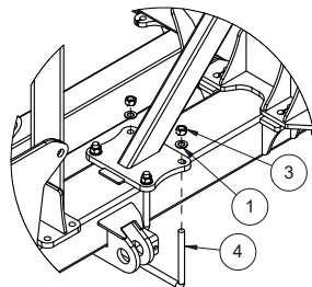
DETAIL H MAIN WING STOP TO BEAM CONNECTION
