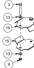
510358 BDL, HANGER - 2 PIPE - DISTRIBUTION
