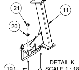
A407740 - WELD, WING STOP - FIFTH FOLD - M80/M90 - BLK
