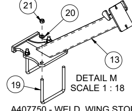
A407750 - WELD, WING STOP - MAIN - M90 - 43" - FRT - BLK
