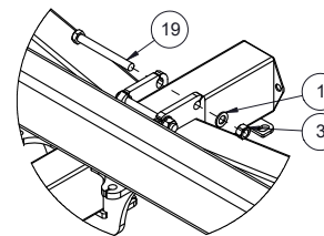
DETAIL O RANK SUPPORT CONNECTION 1 NOTE: IF SUPPORTS DO NOT LINE UP USE RANK SUPPORT CONNECTION 2
