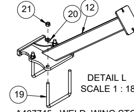
A407745 - WELD, WING STOP - MAIN - M90 - 43" - REAR - BLK
