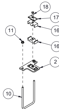
405355 - BAG, HDW - BRIDAL HYD HOSE CLAMP- SM - BL
