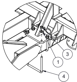
DETAIL A FIFTH FOLD WING STOP TO BEAM CONNECTION
