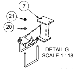
A407715 - WELD, WING STOP - FIFTH FOLD - M60 - BLK
