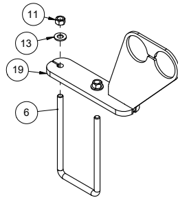
510482 - BDL, PIPE HOLDER - DISTRIBUTION - 6IN - 2 PIPE
