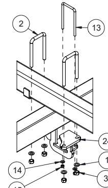
DETAIL J RANK TO WING RAIL LARGE OFFSET CONNECTION
