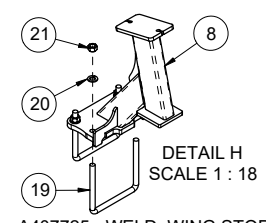
A407725 - WELD, WING STOP - FIFTH FOLD - M80CT - BLK
