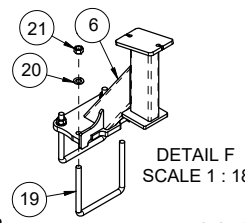
A407710 - WELD, WING STOP - FIFTH FOLD - M60 - BLK
