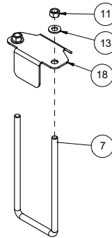
510482 - BDL, PIPE HOLDER - DISTRIBUTION - 6IN - 2 PIPE
