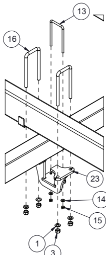
DETAIL G RANK TO MAIN RAIL CONNECTION
