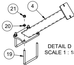
A407700 - WELD, WING STOP - MAIN - M50/M60/M70 - 41 1/4" - FRONT/ REAR - BLK
