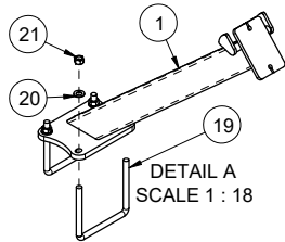
A407780 - WELD, WING STOP - MAIN - M80CT - 45" - FRT - BLK
