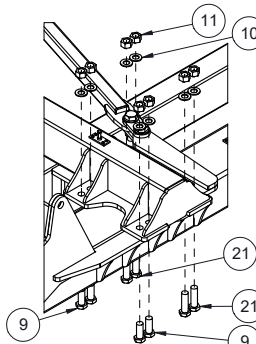
DETAIL I MAIN WING TO WINGBRACE FRONT CONNECTION
