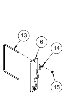
405366 - BAG, HDW - WELD, BOLT ON WIRE LOOPS - MAIN BEAMS - SM - BLK
