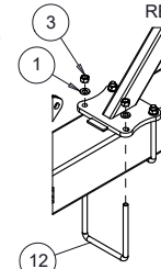
DETAIL P MAIN WING STOP TO REAR BEAM CONNECTION SCALE 1 : 20
