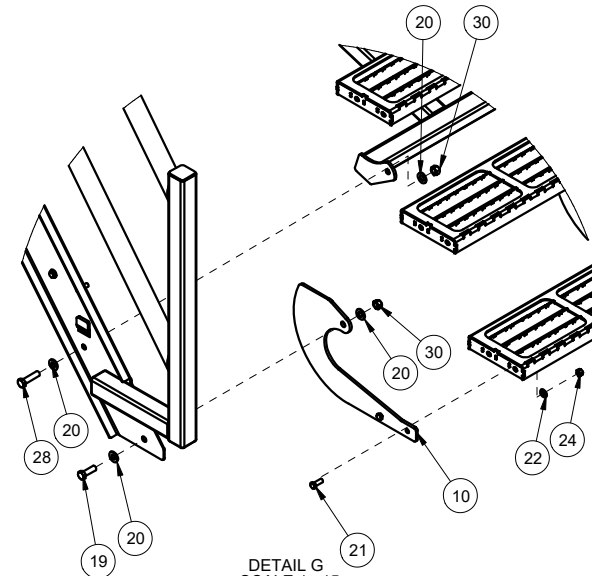
DETAIL G SCALE 1 : 15
