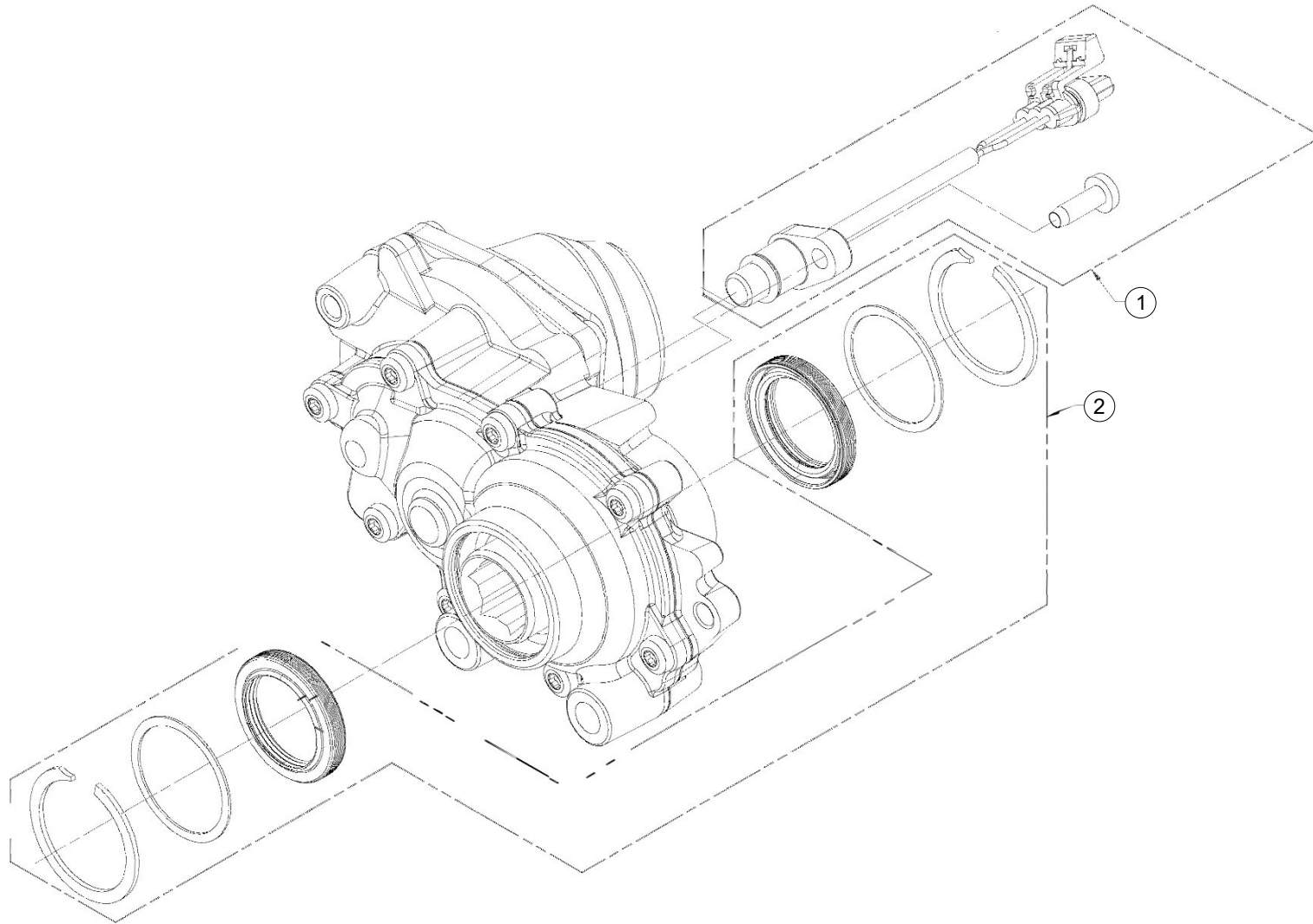
Raven Hydraulic Meter Motor Part Number: 260717
