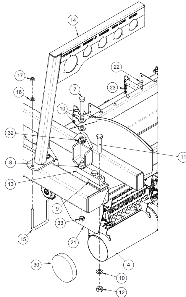
DETAIL B SCALE 1 : 8
