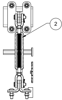
DETAIL BH SCALE 2 : 11
