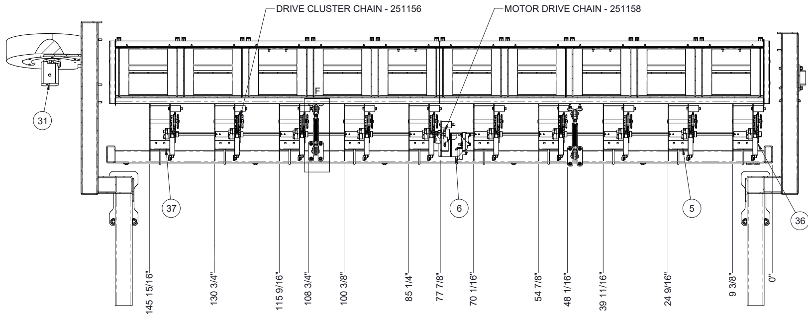
TOP VIEW
