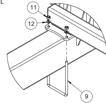
DETAIL C SCALE 1 : 15
