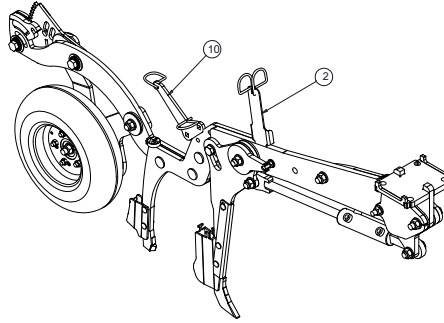
EXAMPLE OF OPENER WITHOUT TRASH WHEEL FRAME
