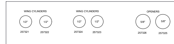
STEEL LINE LAYOUT - REAR OF DRILL STANDING AT FRONT OF DRILL LOOKING TOWARDS REAR
