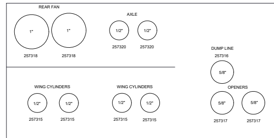
STEEL LINE LAYOUT - FRONT OF DRILL STANDING AT FRONT OF DRILL LOOKING TOWARDS REAR
