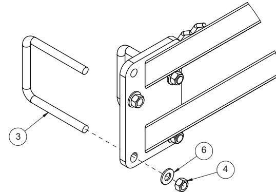
DETAIL B SCALE 1 : 4
