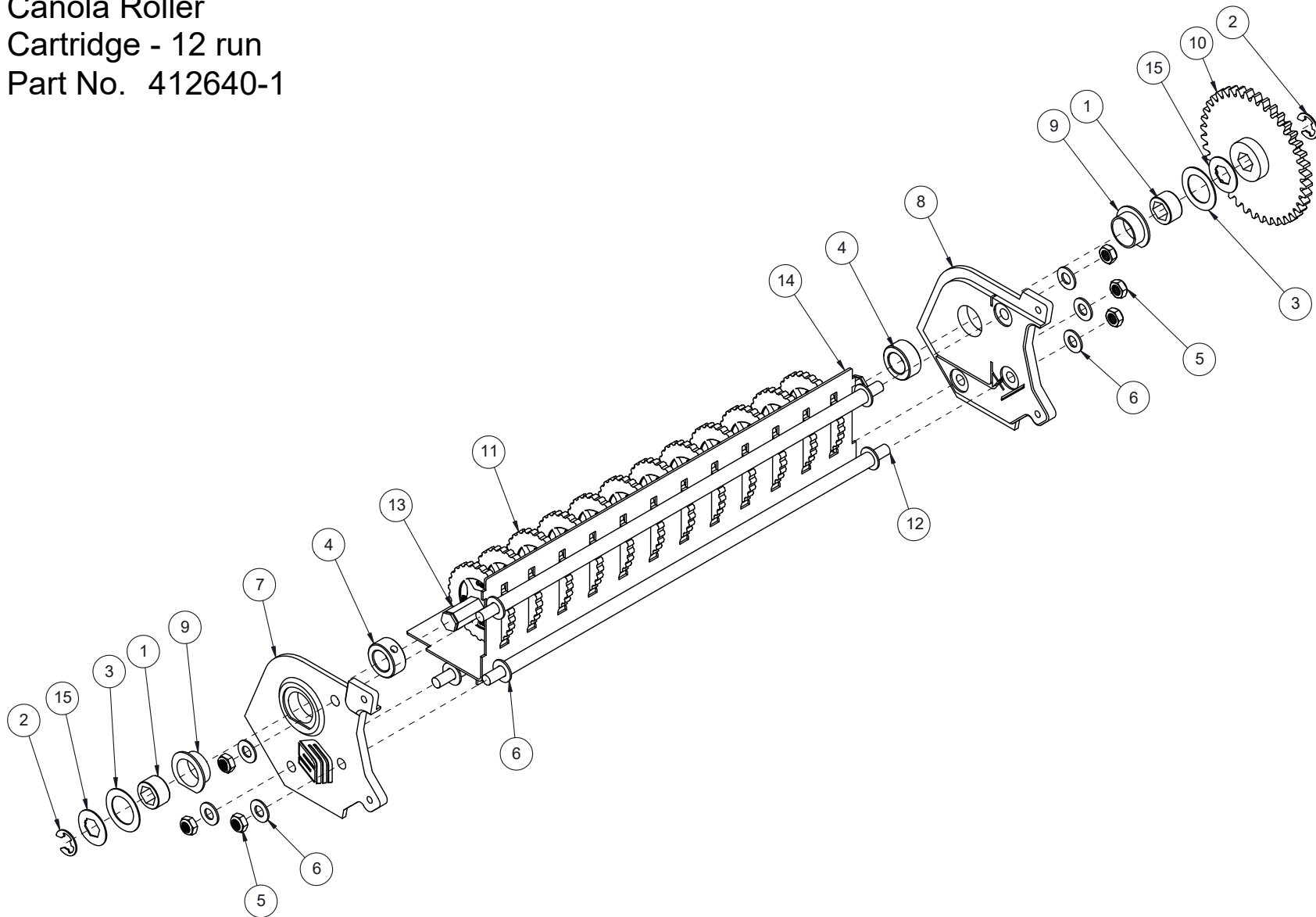
Canola Roller Cartridge - 12 run
