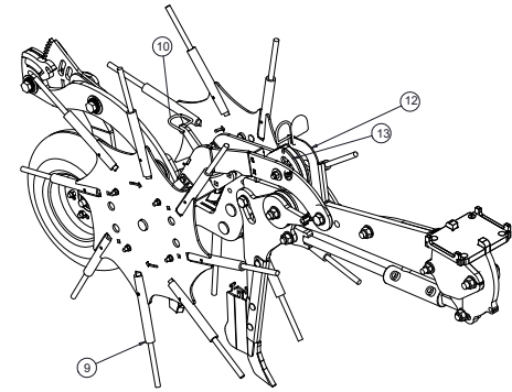
EXAMPLE OF OPENER WITH TRASH WHEEL FRAME NOTE: ALL TRASH WHEELS HAVE THE HEIGHT ADJUST BUNDLE INSTALLED
