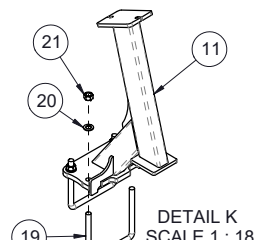
407740 - WELD, WING STOP - FIFTH FOLD - M80/M90 - BLK
