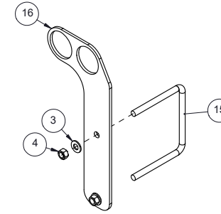
510219 BDL, PIPE HOLDER-DISTRIBUTION - 2 PIPE OFFSET
