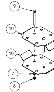
510304 BDL, HANGER-3 PIPE DISTRIBUTION
