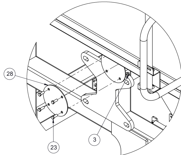
DETAIL B SCALE 1 : 8
