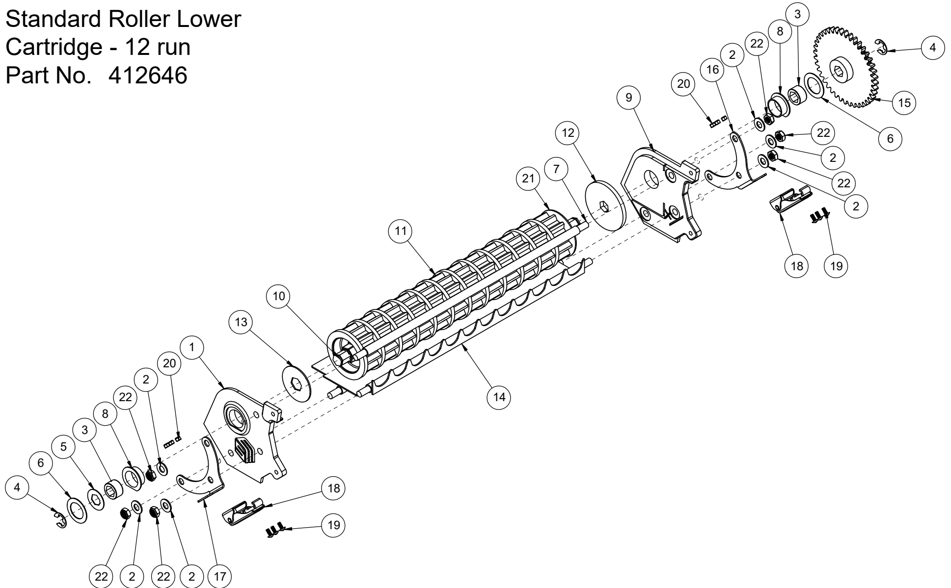
Standard Roller Lower Cartridge - 12 run
