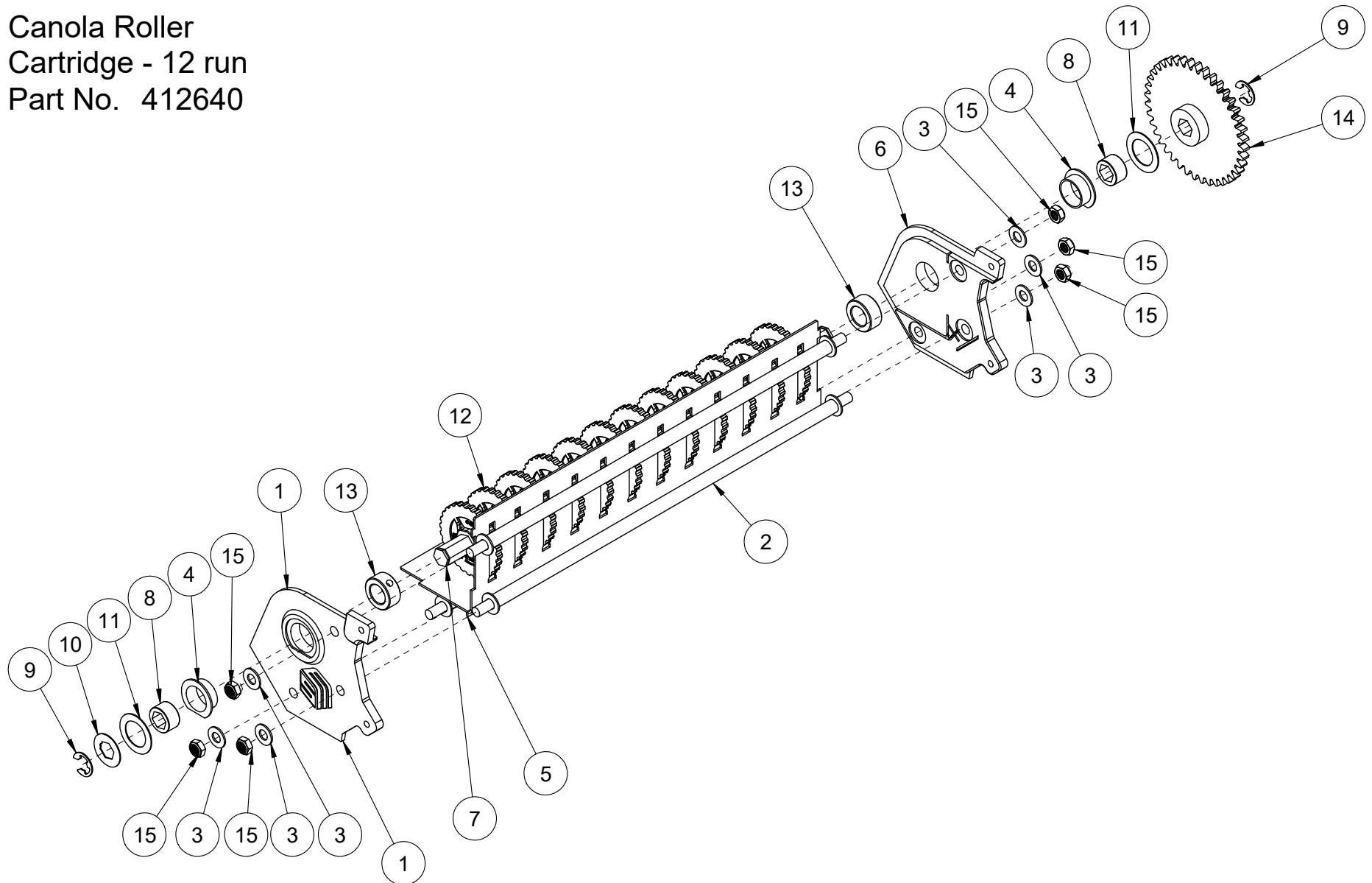
Canola Roller Cartridge - 12 run
