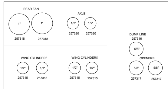
STEEL LINE LAYOUT - FRONT OF DRILL STANDING AT FRONT OF DRILL LOOKING TOWARDS REAR
