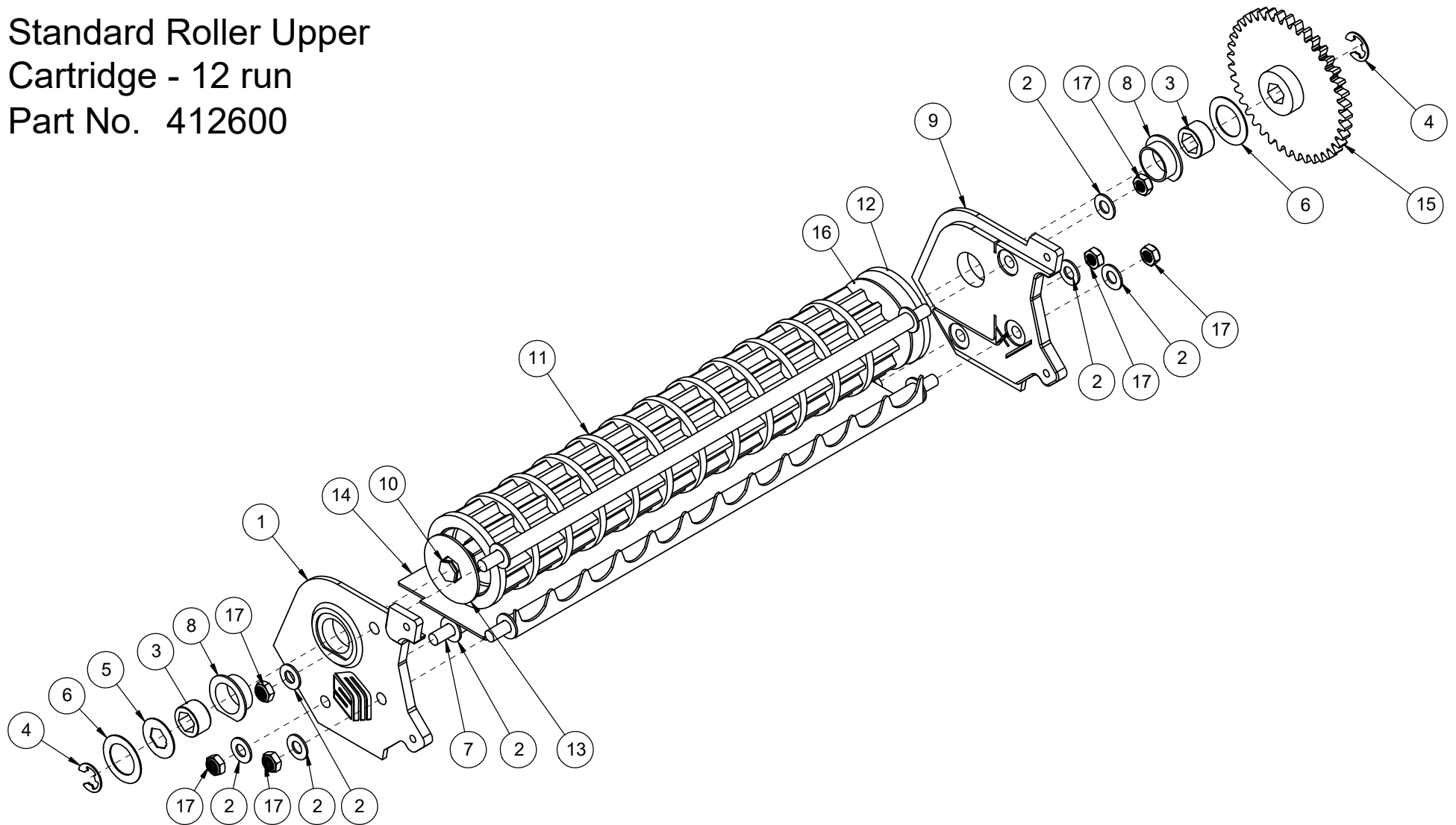
Standard Roller Upper Cartridge - 12 run
