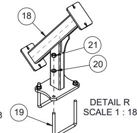
407963 - WELD, WING STOP - 5TH FOLD - BLK
