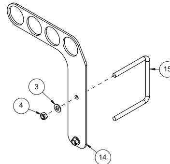
510216 BDL, PIPE HOLDER- DISTRIBUTION - 4 PIPE OFFSET
