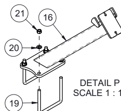
407770 - WELD, WING STOP - MAIN - 40/50CT 3 PLEX - 40" - FRT - BLK
