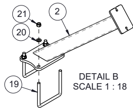
407720 - WELD, WING STOP - MAIN - M80CT - 45" - REAR - BLK
