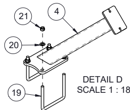
407700-1 - WELD, WING STOP - MAIN - M50/M60/M70 - 41 1/4" - FRONT/ REAR - BLK
