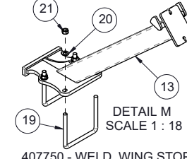
407750 - WELD, WING STOP - MAIN - M90 - 43" - FRT - BLK
