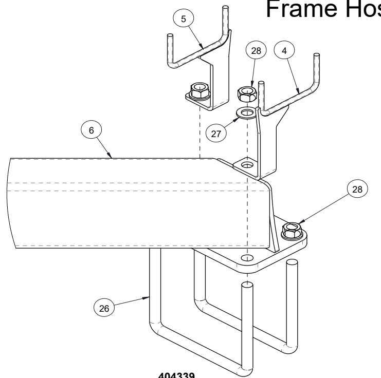
404339 ANGLE BRACKET HOSE HOLDER
