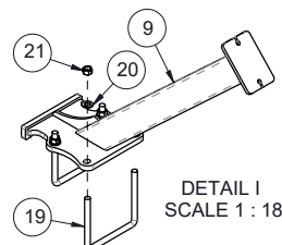
407730 - WELD, WING STOP - MAIN - WIDE M80 - 40 3/8" - FRONT/REAR - BLK
