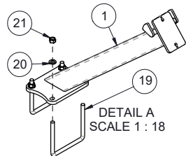
407780 - WELD, WING STOP - MAIN - M80CT - 45" - FRT - BLK
