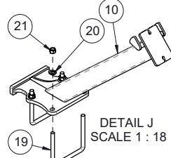
407735 - WELD, WING STOP - MAIN - WIDE M80 - 40 3/8" - FRT - BLK
