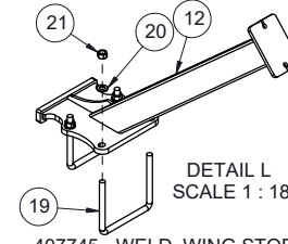
407745 - WELD, WING STOP - MAIN - M90 - 43" - REAR - BLK
