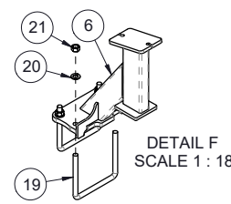
407710 - WELD, WING STOP - FIFTH FOLD - M60 - BLK
