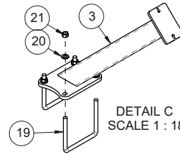
407615-1 - WELD, WING STOP - MAIN - 40/50CT 3 PLEX - 40" - REAR - BLK
