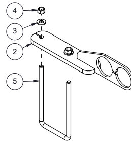
510309 - BDL, PIPE HOLDER - 2 PIPE
