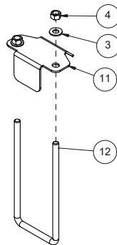
510338 BDL, HANGER - SINGLE PIPE - DISTRIBUTION
