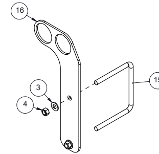
510304 BDL, HANGER-3 PIPE DISTRIBUTION
