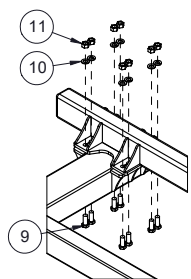
DETAIL M WING RAIL TO BEAM CONNECTION
