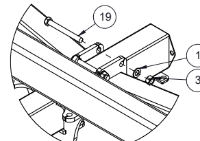
DETAIL O RANK SUPPORT CONNECTION 1 NOTE: IF SUPPORTS DO NOT LINE UP USE RANK SUPPORT CONNECTION 2
