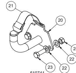
510741 BDL, PIPE HOLDER - DISTRIBUTION - 6IN - 2 PIPE
