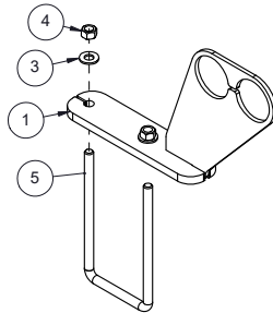
510314 - BDL, PIPE HOLDER - 6IN - 2 PIPE
