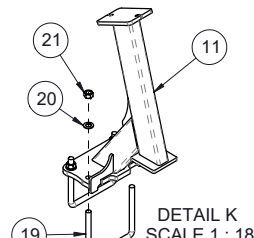
407740 - WELD, WING STOP - FIFTH FOLD - M80/M90 - BLK
