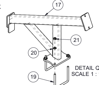
407977 - WELD, WING STOP - STD 5 PLEX - REAR - BLK
