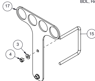
510318 - BDL, PIPE HOLDER - DISTRIBUTION - 4 PIPE - CENTER
