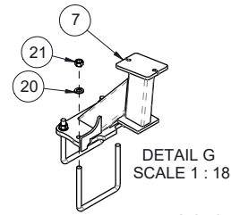
407715 - WELD, WING STOP - FIFTH FOLD - M60 - BLK
