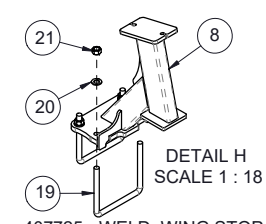
407725 - WELD, WING STOP - FIFTH FOLD - M80CT - BLK
