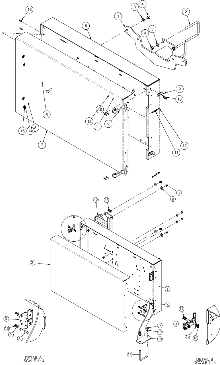
BDL, AIR/ELEC CONTROL HOUSING - UPII 530 (406471-1)
