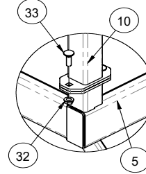
DETAIL C SCALE 1 : 8
