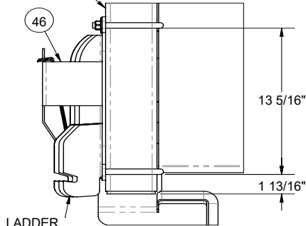
DETAIL E SCALE 1 : 6
