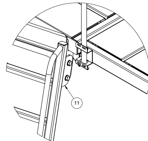
DETAIL K SCALE 1 : 10
