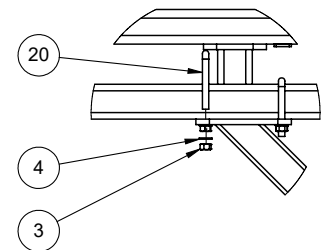
DETAIL T SCALE 2 : 35
