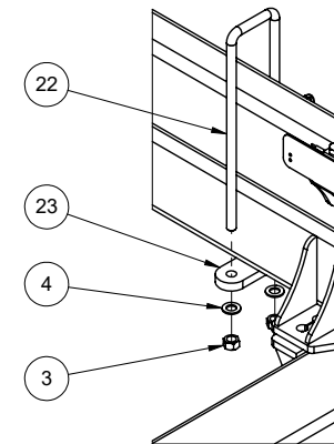
DETAIL U SCALE 2 : 25
