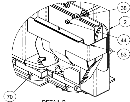
DETAIL B SCALE 1 : 8
