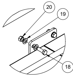
DETAIL I SCALE 1 : 10
