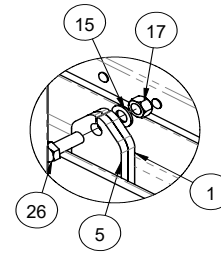
DETAIL D SCALE 1 : 8
