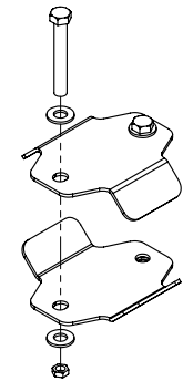
510358 - BDL - HANGER - 2 PIPE - DISTRIBUTION
