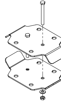
510304 - BDL - HANGER - 3 PIPE - DISTRIBUTION
