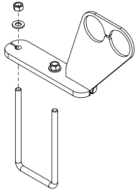
510314 - BDL, PIPE HOLDER - DISTRIBUTION - 6IN - 2 PIPE
