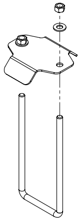
510302 - BDL - HANGER - 2 PIPE - DISTRIBUTION
