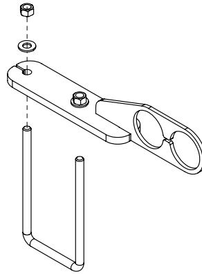
510309 - BDL, PIPE HOLDER - DISTRIBUTION - 2 PIPE
