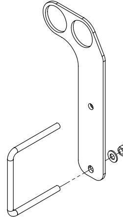
510219 - BDL, PIPE HOLDER - DISTRIBUTION - 2 PIPE - OFFSET
