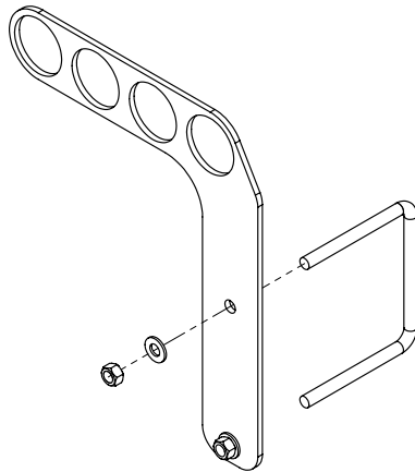
510216 - BDL, PIPE HOLDER - DISTRIBUTION - 4 PIPE - OFFSET
