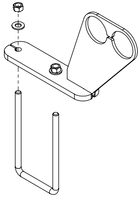
510314 - BDL, PIPE HOLDER - DISTRIBUTION - 6IN - 2 PIPE
