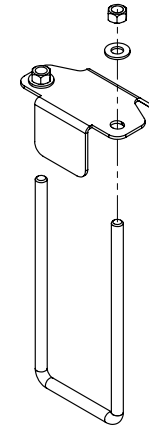
510338 - BDL - HANGER - SINGLE PIPE - DISTRIBUTION
