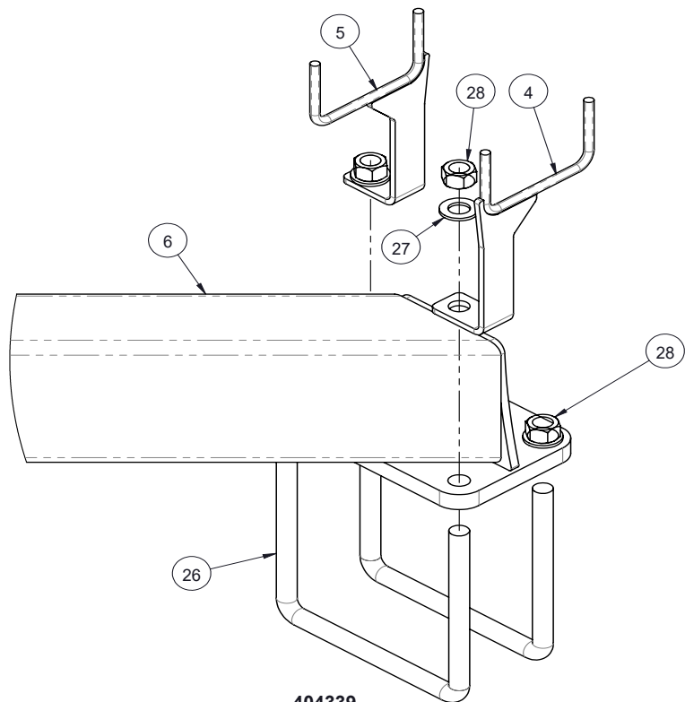
404339 ANGLE BRACKET HOSE HOLDER
