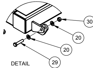
DETAIL SCALE 1 : 12
