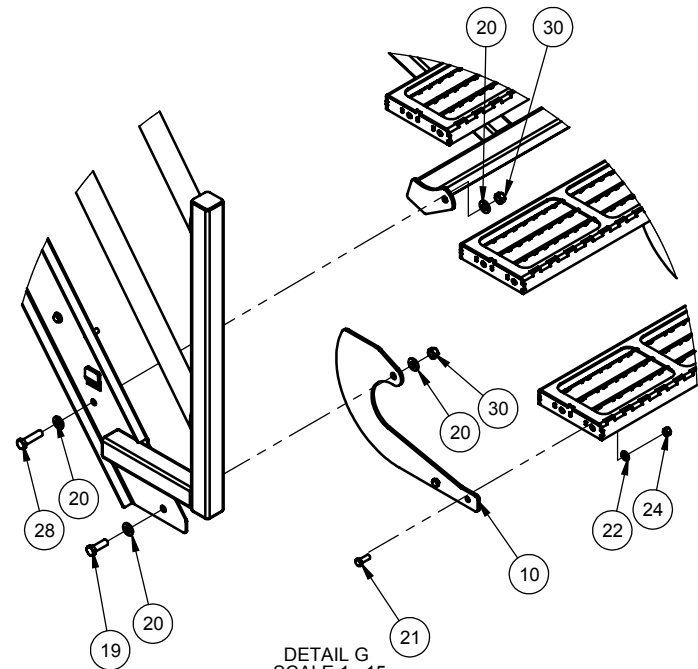
DETAIL G SCALE 1 : 15
