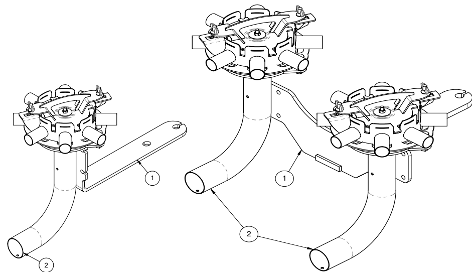
8 OUTLET - DUAL SHOOT MOUNT
