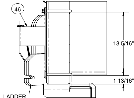
DETAIL E SCALE 1 : 6
