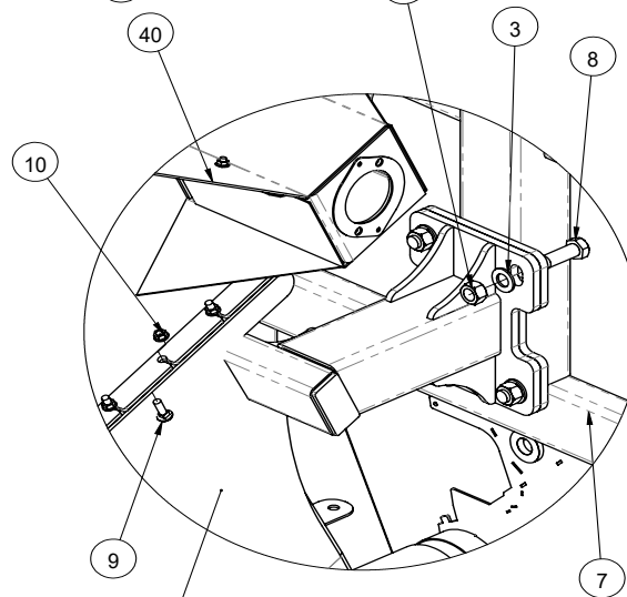
DETAIL F SCALE 1 : 8
