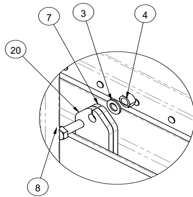
DETAIL A SCALE 1 : 6
