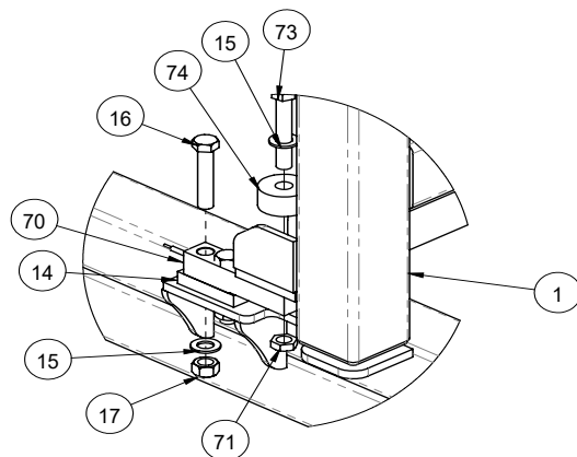
DETAIL H SCALE 1 : 8
