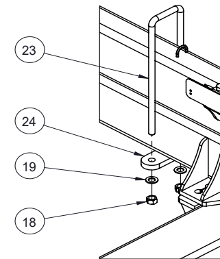
DETAIL U SCALE 2 : 25
