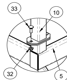
DETAIL C SCALE 1 : 8
