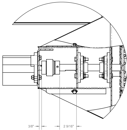
DETAIL A SCALE 1:4 NOTE: COUPLER INSTALLATION DETAIL
