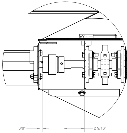
DETAIL A SCALE 1:4 NOTE: COUPLER INSTALLATION DETAIL
