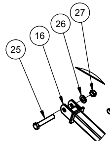
DETAIL E SCALE 1 : 15
