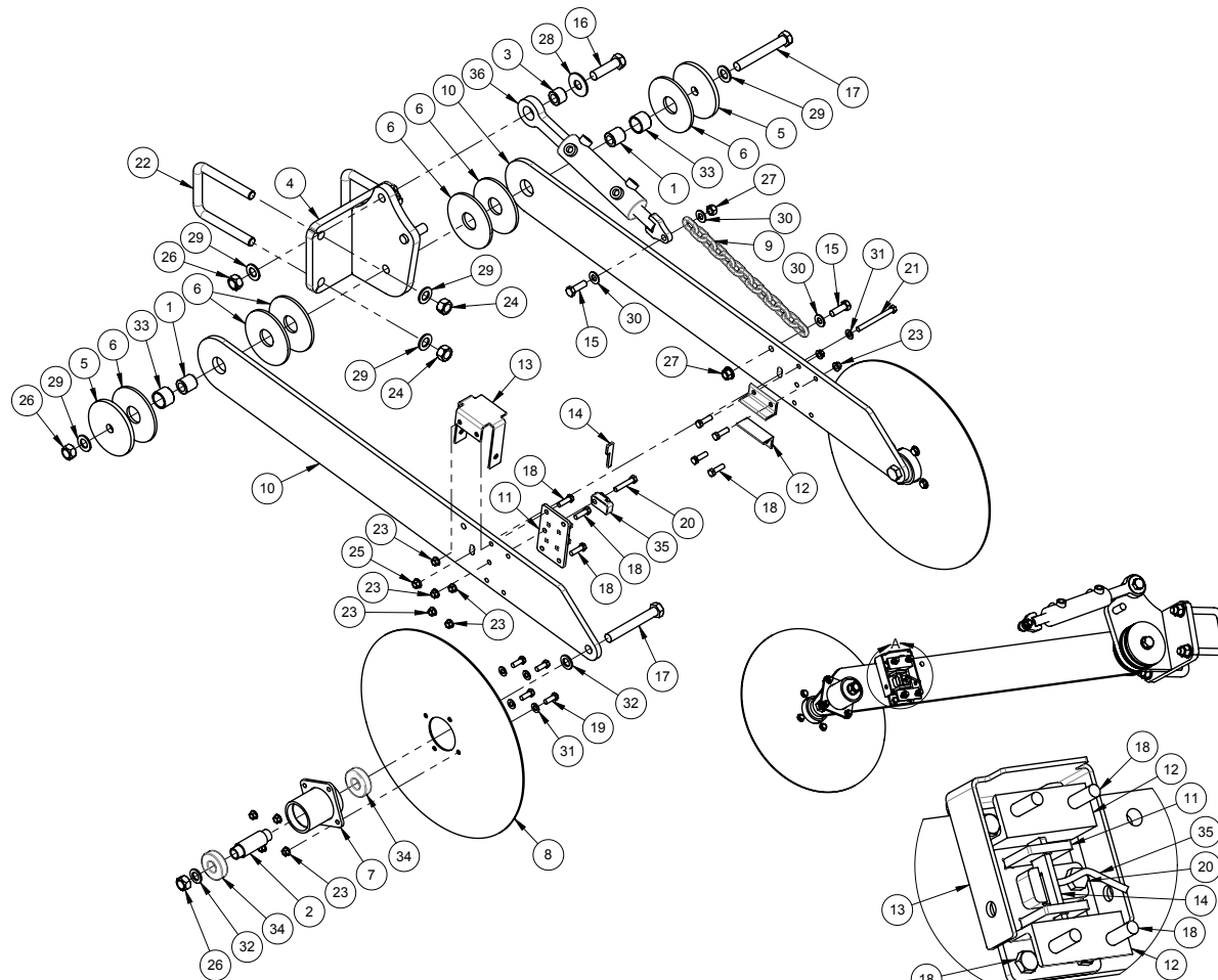
HALL EFFECT SENSOR ASSEMBLY SOME PARTS NOT SHOWN FOR CLARITY
