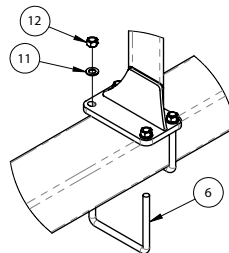
ANGLE BRACKET TO BEAM CONNECTION
