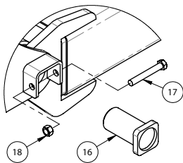
HINGE PIN CONNECTION
