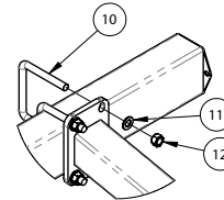
RANK SUPPORT CONNECTION 2
