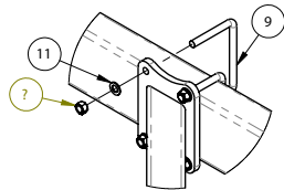
ANGLE BRACKET TO RAIL CONNECTION
