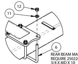
MAIN WING STOP TO BEAM CONNECTION
