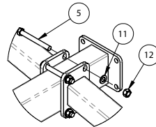
RANK SUPPORT CONNECTION 1 (IF SUPPORTS DO NOT LINE UP USE RANK SUPPORT CONNECTION 2)
