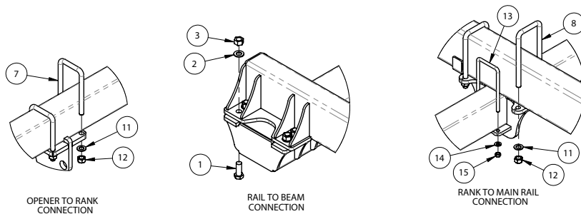
OPENER TO RANK CONNECTION
