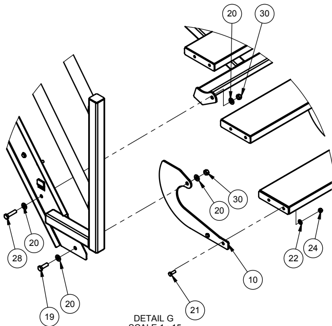
DETAIL G SCALE 1 : 15
