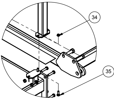
DETAIL F SCALE 1 : 15
