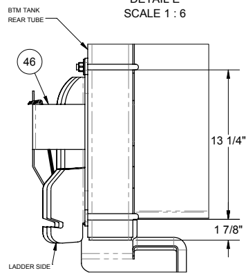
U-BOLT LOCATION FOR TRAYS AND GATES
