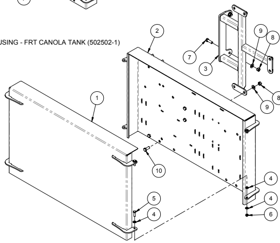
BDL AIR/ELEC CONTROL HOUSING - SXX (405950)
