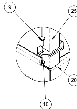
DETAIL C SCALE 1 : 6
