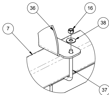
DETAIL E SCALE 1 : 6
