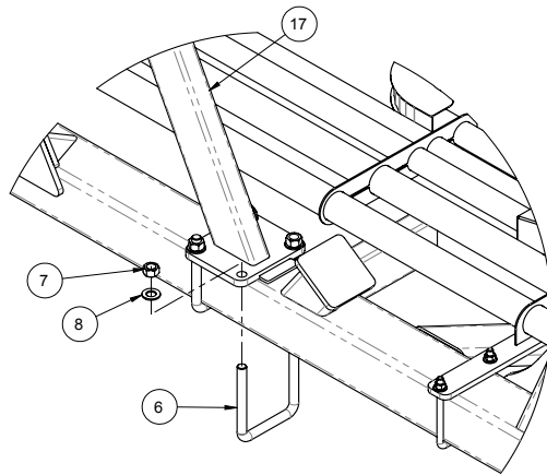
WING STOP MOUNTS FOR MAIN WING
