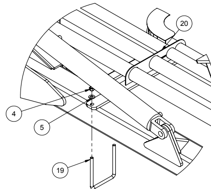
DISTRIBUTION PIPE MOUNTS
