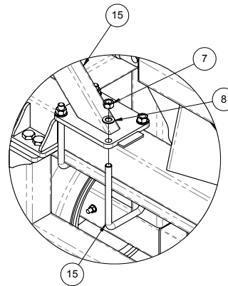
WING STOP MOUNT FOR MAIN FRAME
