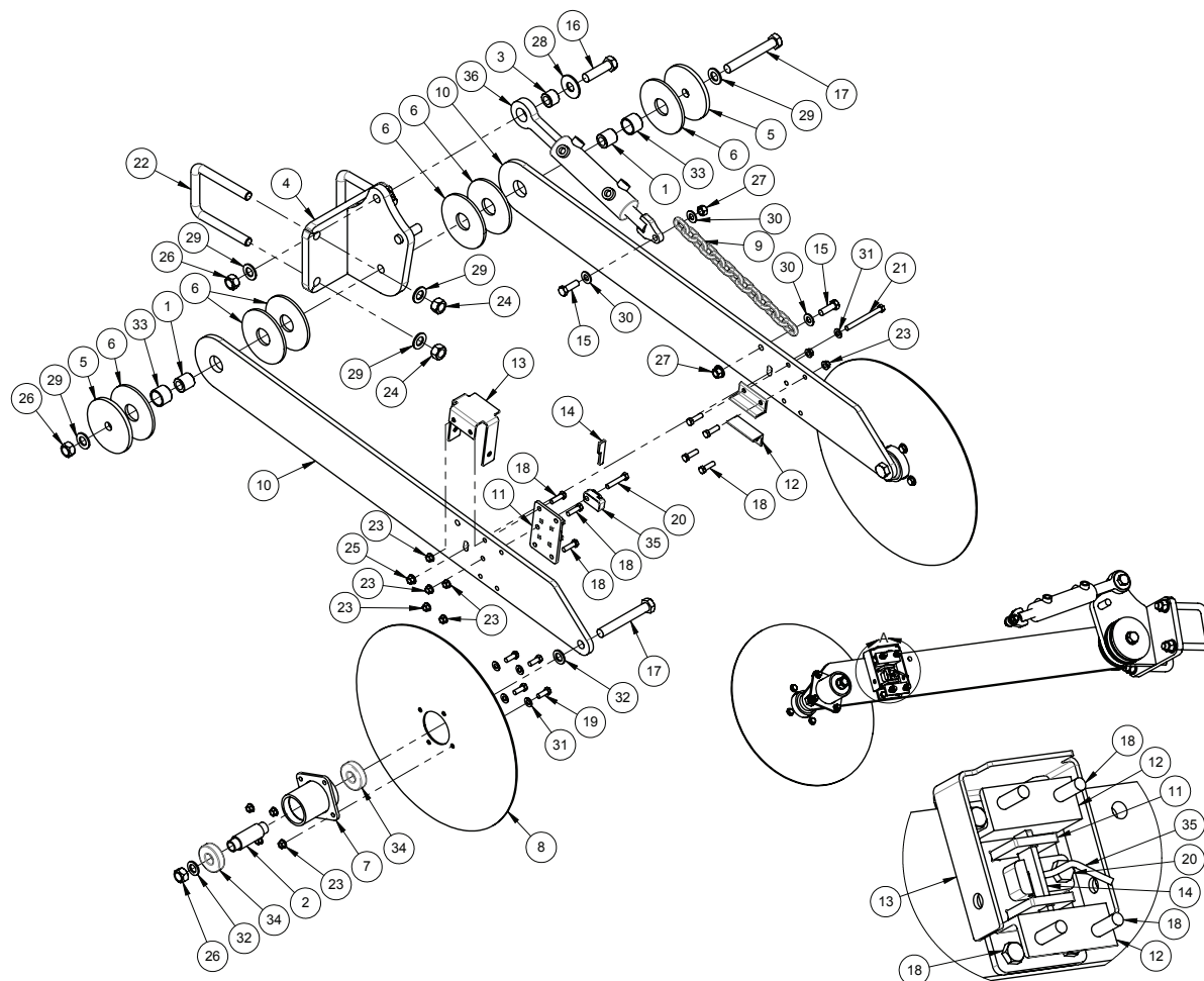
HALL EFFECTS SENSOR ASSEMBLY SOME PARTS NOT SHOWN FOR CLARITY
