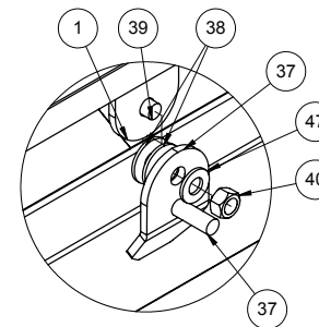
DETAIL J SCALE 1 : 4
