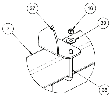
DETAIL E SCALE 1 : 6
