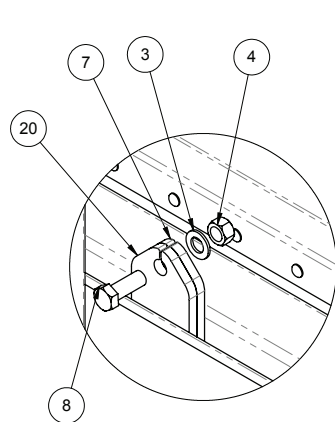
DETAIL A SCALE 1 : 6
