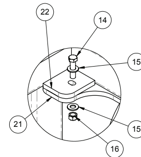
DETAIL D SCALE 1 : 6
