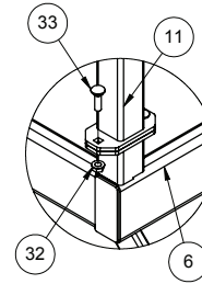
DETAIL C SCALE 1 : 8
