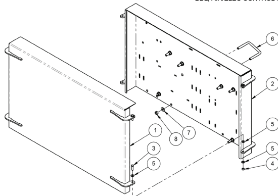
BDL, AIR/ELEC CONTROL HOUSING - SXX045 (410445)
