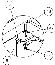
DETAIL E SCALE 1 : 8
