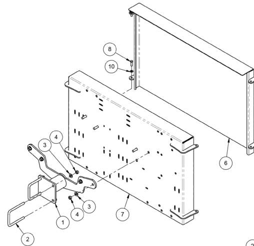
BDL, AIR/ELEC CONTROL HOUSING - FRT CANOLA TANK (502502-1)
