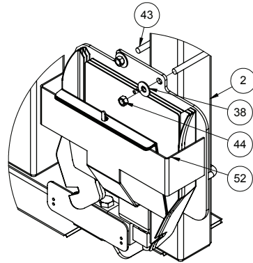
DETAIL B SCALE 1 : 8
