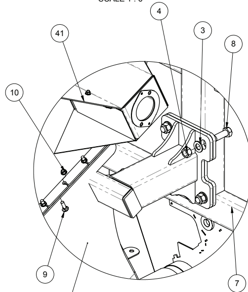
DETAIL F SCALE 1 : 8
