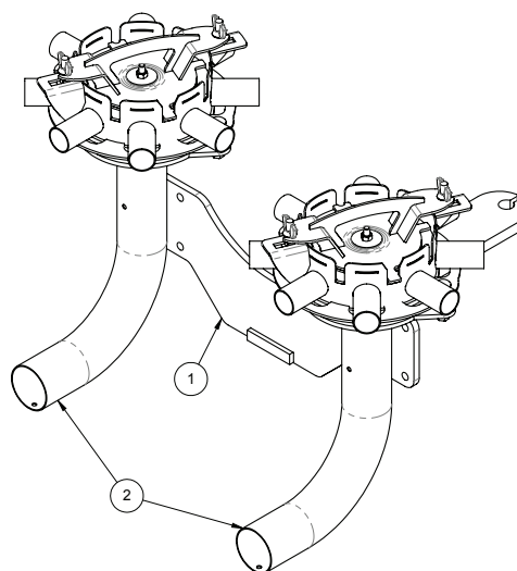
8 OUTLET - DUAL SHOOT MOUNT
