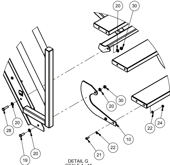
DETAIL G SCALE 1 : 15
