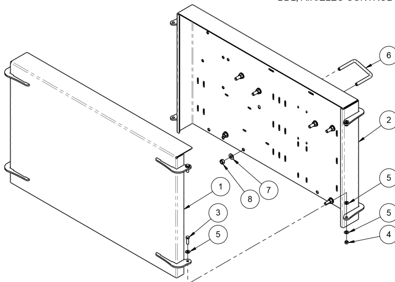
BDL, AIR/ELEC CONTROL HOUSING - SXX045 (410445)
