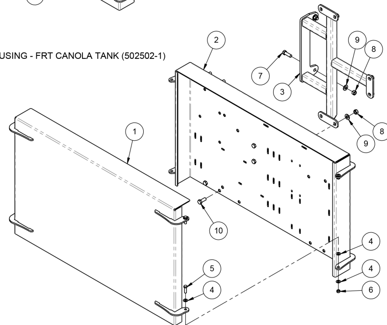
BDL, AIR/ELEC CONTROL HOUSING - SXX (405950)
