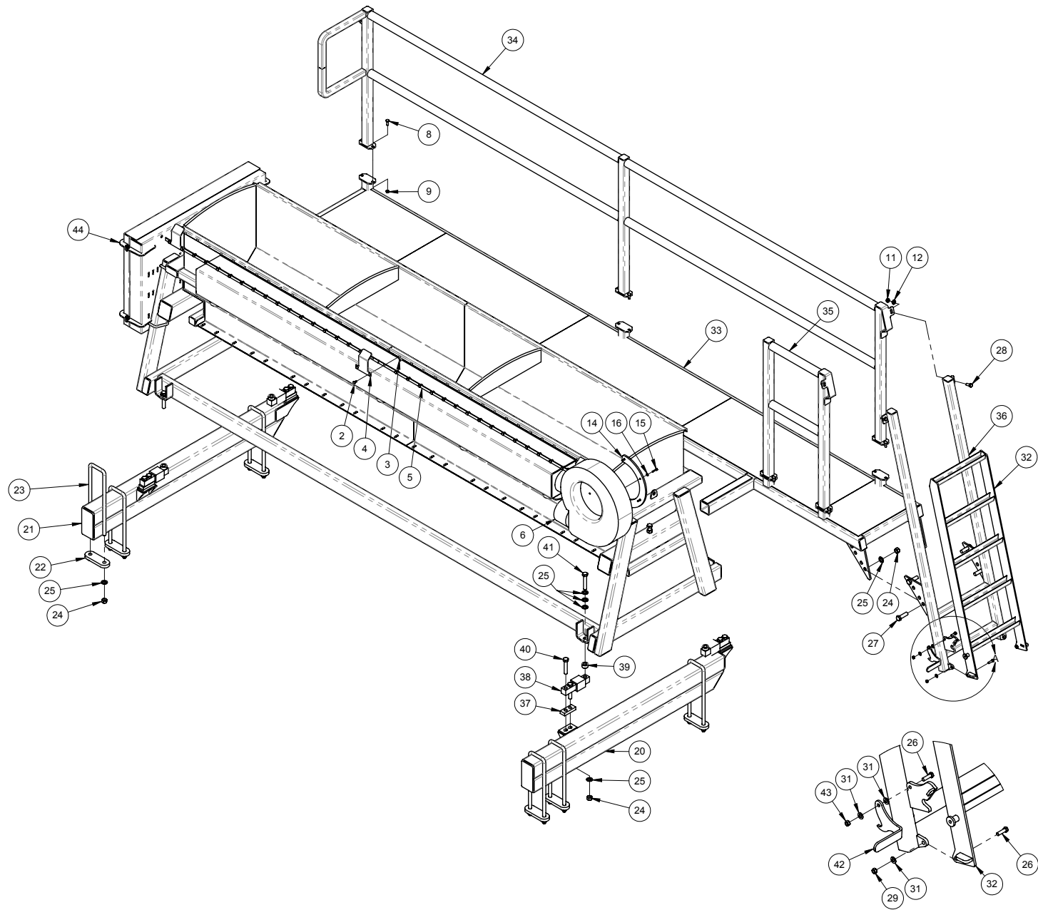
DETAIL A SCALE 1 : 12
