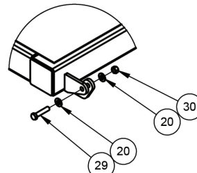
DETAIL D SCALE 1 : 15
