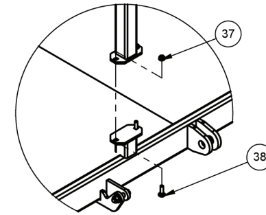
DETAIL F SCALE 1 : 15
