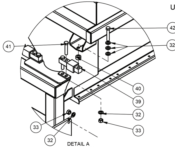
DETAIL A SCALE 1 : 15
