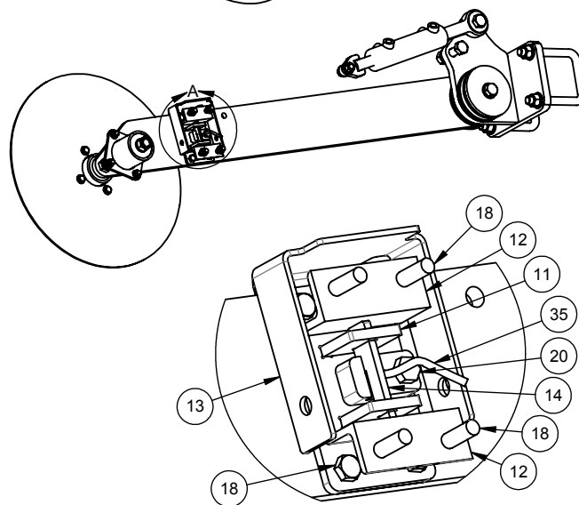
HALL EFFECTS SENSOR ASSEMBLY SOME PARTS NOT SHOWN FOR CLARITY
