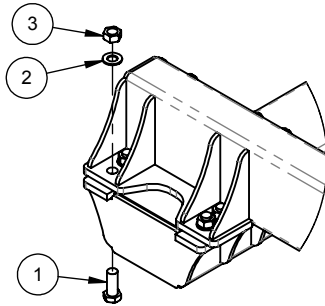
RAIL TO BEAM CONNECTION
