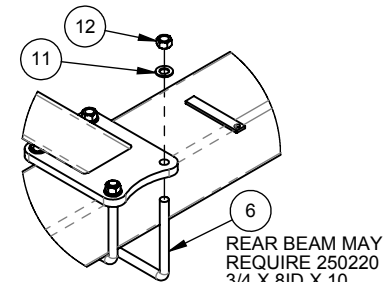
MAIN WING STOP TO BEAM CONNECTION
