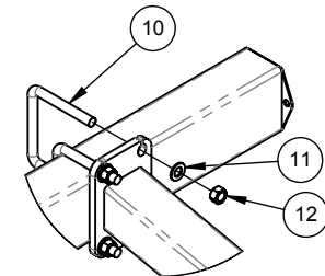
RANK SUPPORT CONNECTION 2
