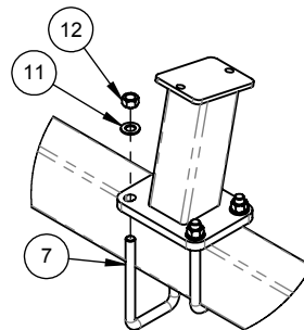
FIFTH FOLD WING STOP TO RAIL TOP CONNECTION
