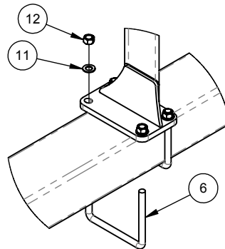
ANGLE BRACKET TO BEAM CONNECTION
