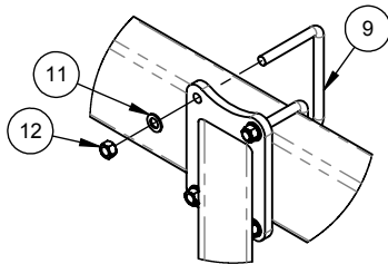
ANGLE BRACKET TO RAIL CONNECTION
