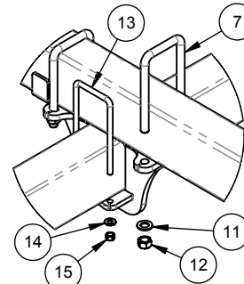
RANK TO WING RAIL CONNECTION
