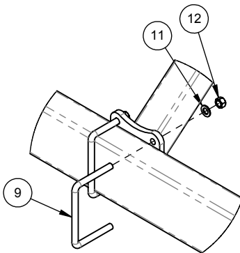
MAIN WING STOP TO RAIL SIDE CONNECTION
