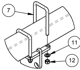
OPENER TO RANK CONNECTION
