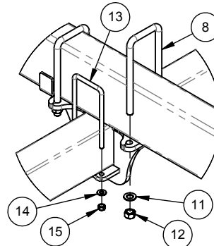
RANK TO MAIN RAIL CONNECTION
