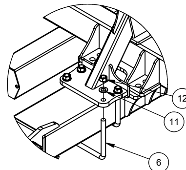
FIFTH FOLD WING STOP TO BEAM CONNECTION
