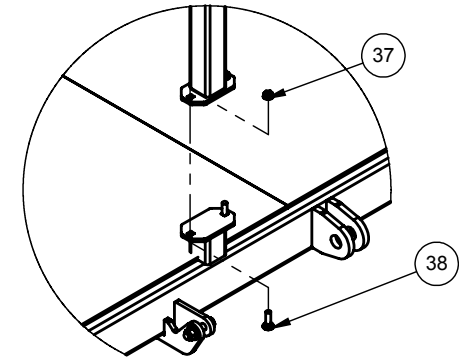
DETAIL F SCALE 1 : 15
