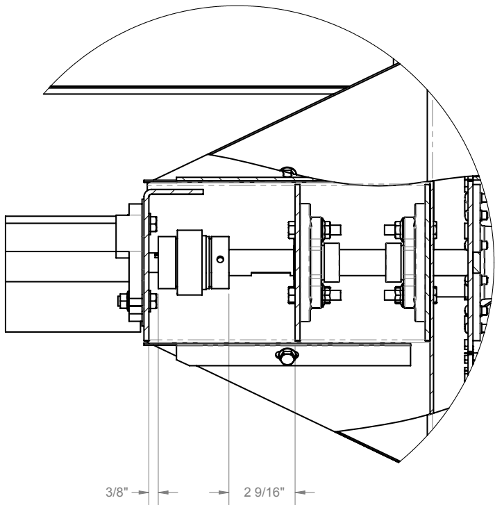
DETAIL A SCALE 1 : 4 NOTE: COUPLER INSTALLATION DETAIL
